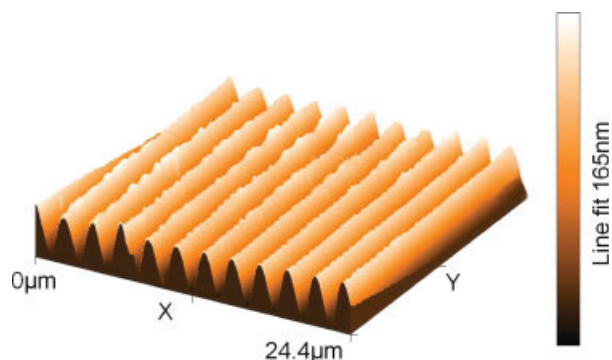
Figure 11. Atomic force microscope scan of the diffraction grating recorded in a film ( 24 \times 24.4 \mu\text{m}^2 ) of (uracil) 16 -[G-2]-PAMAM, 7 . [Color figure can be viewed in the online issue, which is available at www.interscience.wiley.com .]
