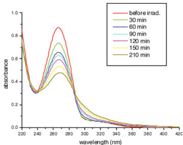
Figure 8. Absorption spectrum of an (uracil) 8 -[G-1]-PAMAM, 6 , film before and after irradiated at 257 nm, with a low intensity power source ( <0.5 \text{ mW/cm}^2 ), an isosbestic point is observed at 286 nm.
